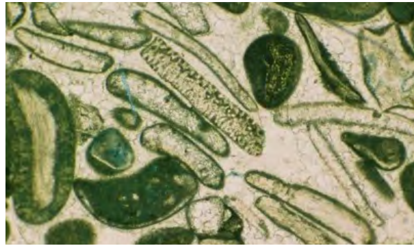
Fig. 12a Effects of large calcite cement crystals growing across grain boundaries. a, the edges of formerly aragonite shell fragments are usually represented by microporous lines of weakness where lines of small seed crystals run along the junction of the primary and the secondary (biomouldic) porosity (the micrite envelope). b, if some crushing took place after the aragonite dissolution but before the start of spar growth, then the micrite envelopes became broken and discontinuous. This allowed a stronger fabric of larger calcite crystals to cross through the gaps from primary to secondary porosity and hence interrupt the weak zone that run along the edges of the grains. This fabric is often seen in the shellier Lincs Limestone and Inferior Oolite freestones.
