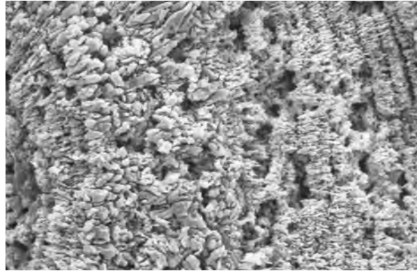
Fig. 3d Microporosity within the cortex of a single oolith, Coombe Down Stone, Bath.
