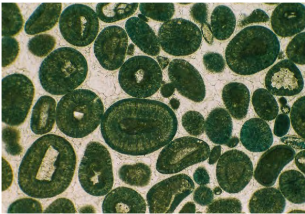
Fig. 11 Reduction of microporosity within ooliths in many Lincs Limestone and Inferior Oolite freestones by development of a fabric of radial calcite crystals in the oolith cortices.
