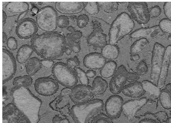
Fig. 3 Macroporosity ( >5\mu\text{m} ) (a, b) and microporosity ( <5\mu\text{m} ) (c, d) in Jurassic limestone freestones shown in Scanning Electron Micrographs. Fig. 3a Weldon Stone with thin layer of calcite cement coating surface of grains, and large volumes of well-connected pore-space (filled with resin in this sample) remaining.
