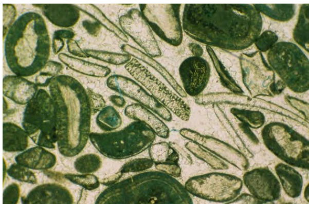
Fig. 6 Typical texture of Bath Stone seen in thin-section. Ooliths and shell fragments touch at point contacts; intergranular and secondary macroporosity are completely filled by calcite spar. This example is Box Ground Stone, which has well-developed layers of shell debris.
