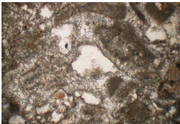
Fig. 14 Thin section of Dundry stone. The clear white areas are regions of uncemented macroporosity.
